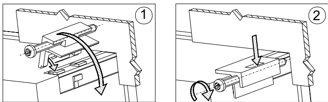
Fig. 2. Meter fixing.
