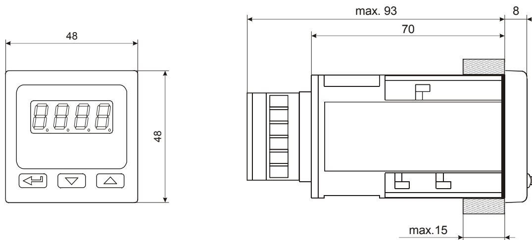
Fig. 2. Controller dimensions.
