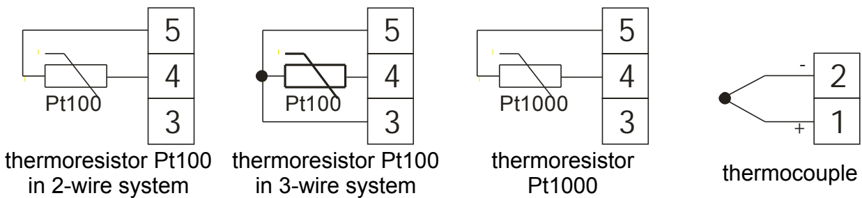
Fig. 4. Input signals
